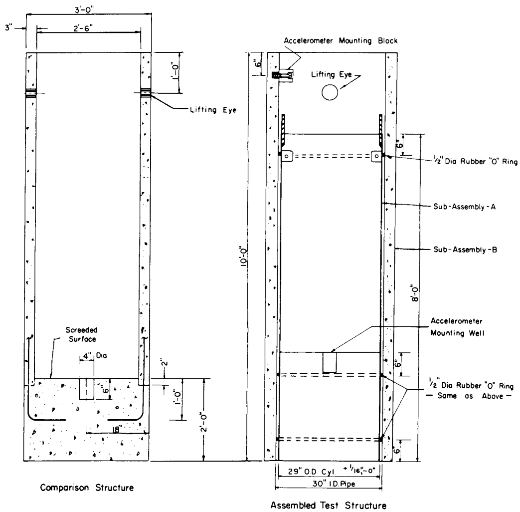
Fig. 2—Comparison structure and test structure.
